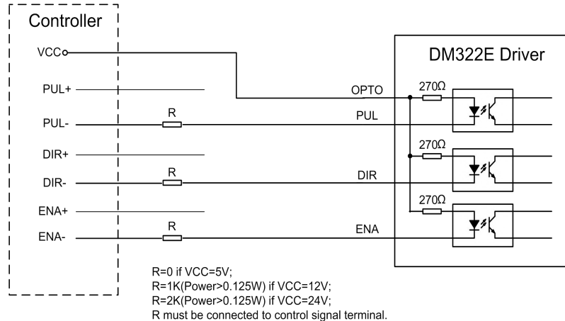
Figure 3: Connections to difference control signal
