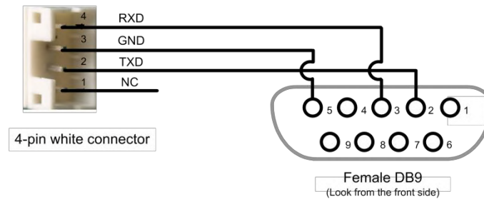
Figure 3: CABLE-PC-1 connectors
