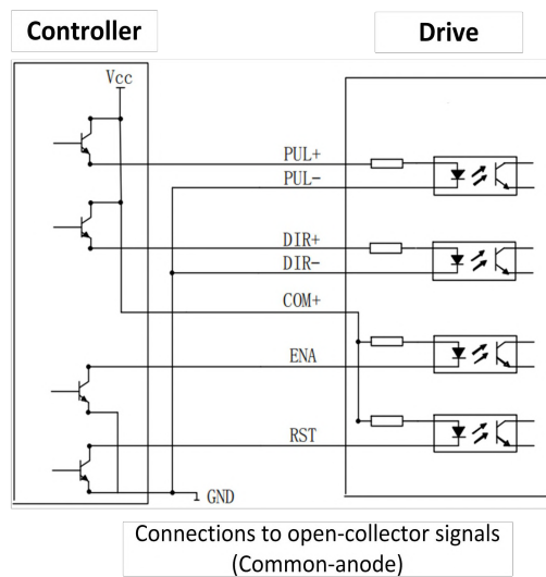
Figure 6: Digital input connections
